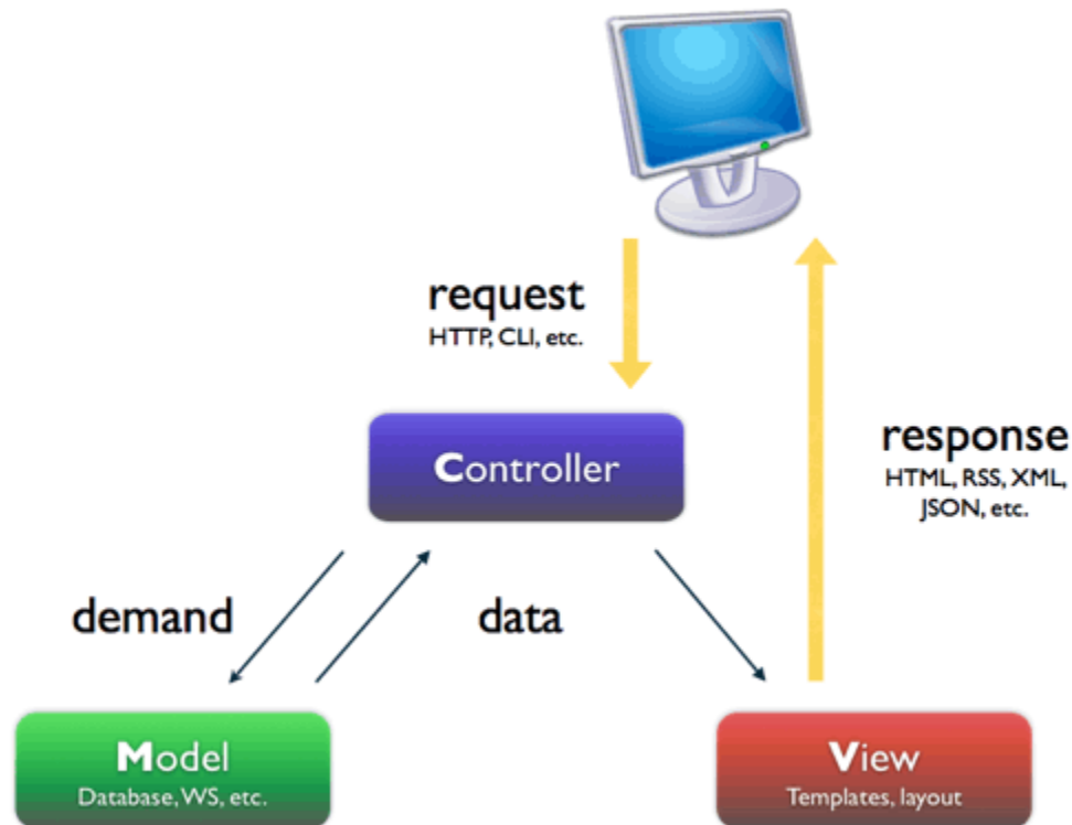
Fig.1. Code Igniter Framework
