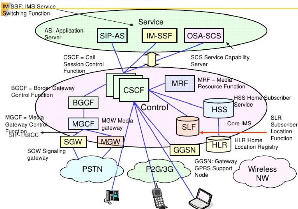
Fig.4. Software architecture of—IMS
